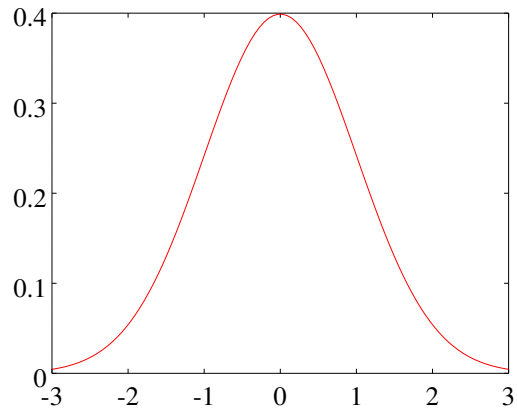
Figure 1: Plot of the standard Gaussian density.
