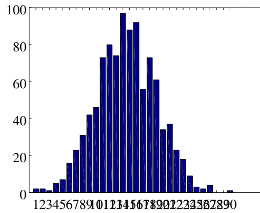
Figure 2: Histogram of 1000 samples from the standard Gaussian density.
